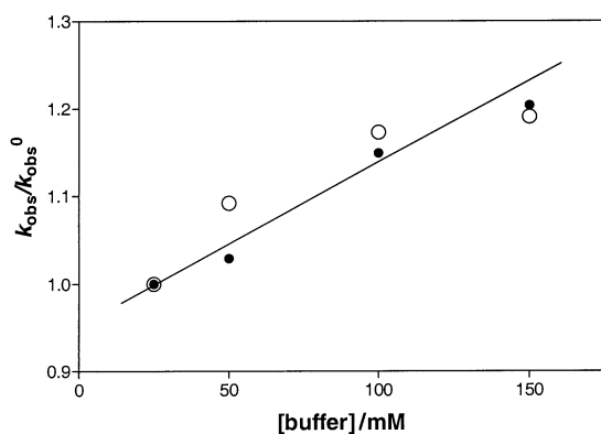
Fig. 1 Effect of acetic acid buffer (buffer ratio 9:1) on the rate of solvolysis of 1-OH (○) and 1-OMe (●) in 50 vol% methanol in water at 25 °C; 0.25 M sodium perchlorate added.
